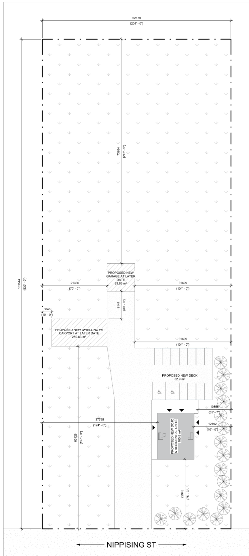
SITE PLAN 1" = 30'-0"
